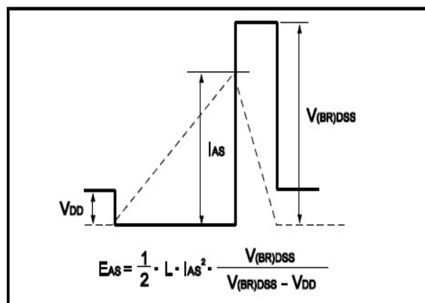
Fig.12 Avalanche Waveform
